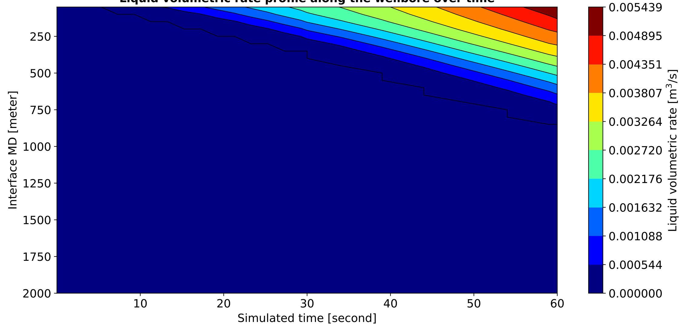
Liquid volumetric rate profile along the wellbore over time
